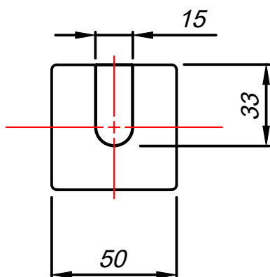
Mounting Plate
