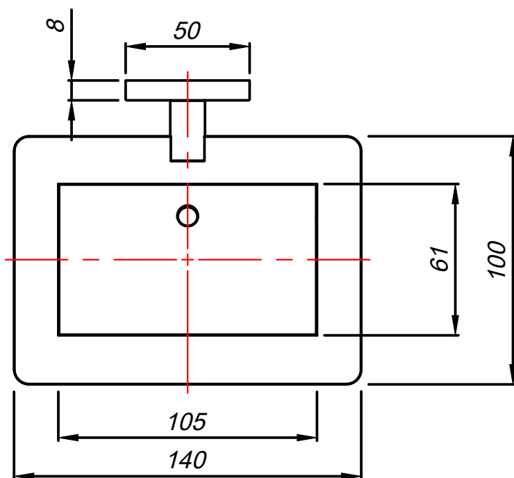
Mounting Plate
